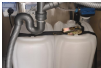
25L clean water tank & 25L waste water tank
