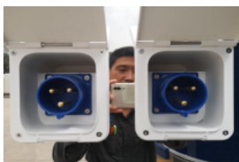
2 x outside power inlets (16A or 32A)
