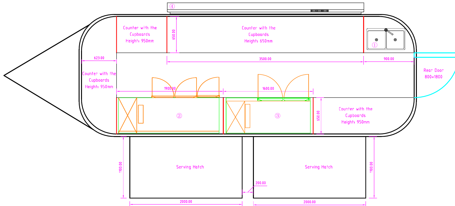
6m Shiny Airstream Food Trailer Inside Layout
